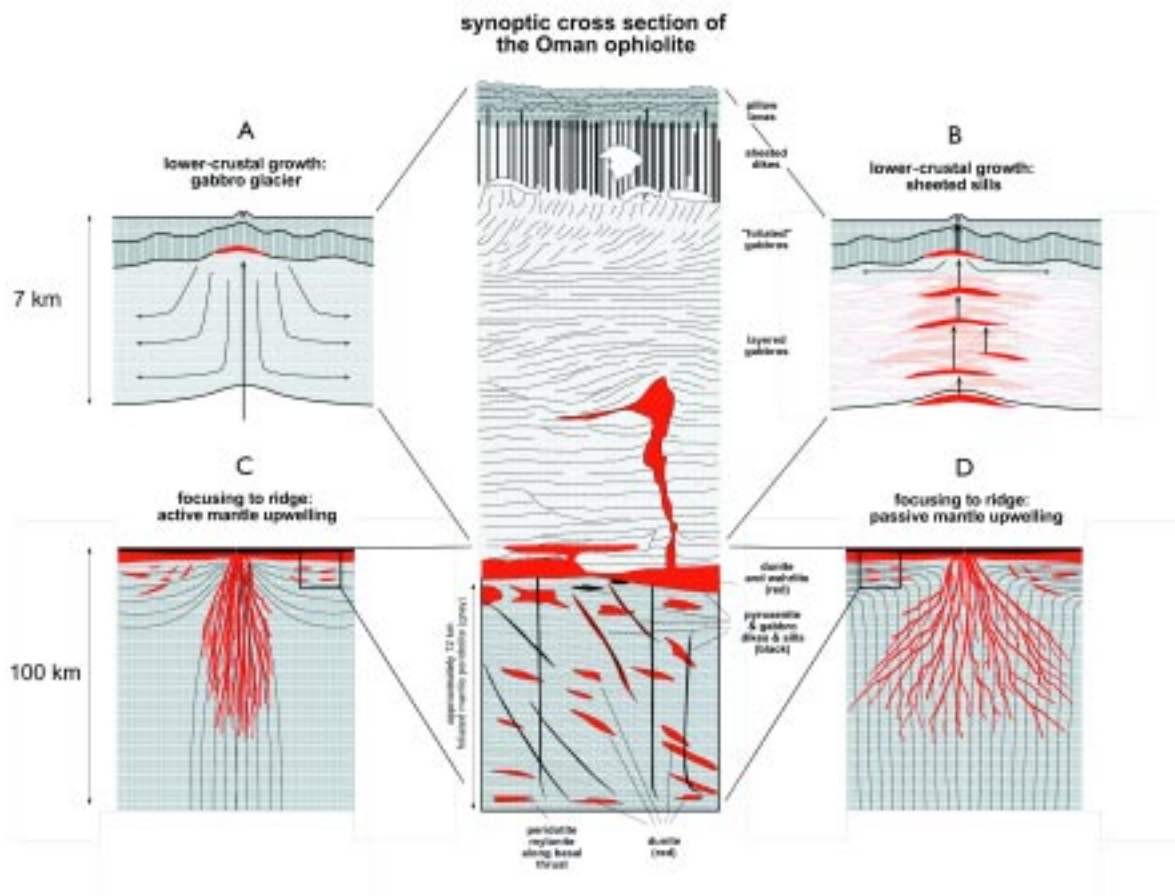
Figure 33. End-member models for igneous accretion of the lower crust at fast-spreading mid-ocean ridges and for focusing of melt extraction in the mantle from a ~100 km wide melting region to a ~10 km wide crustal accretion zone beneath the ridge axis. (A) "Gabbro glacier" model. Ductile flow downward and outward from a single, shallow axial magma chamber forms the entire lower crust. (B) "Sheeted sill" model. Melt transport by hydrofracture and in situ emplacement of the lower crust by sill intrusions. Most gabbros are crystallized at their current depth of emplacement. (C) Focused solid mantle upwelling, resulting from buoyancy driven mantle convection, mainly vertical melt transport. (D) Passive solid mantle upwelling, resulting from plate spreading, with coalescing melt flow conduits. Central panel is a summary cross-section of the Oman ophiolite, where upper mantle and lower crustal exposures allow testing of these hypotheses. Figure reprinted by permission from Nature, Kelemen, P.B. et al., Extraction of mid-ocean ridge basalt from the upwelling mantle by focused flow of melt in dunite channels, 375, Figure 1, p.748, copyright 1995 Macmillan Magazines Ltd.
