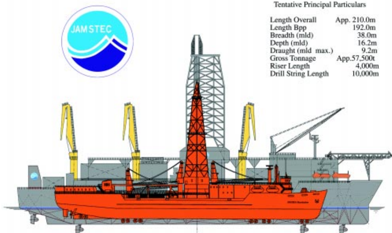
Figure 37. Silhouettes of ships representing the two primary drilling platforms to be used in the IODP. In the foreground is a silhouette of the JOIDES Resolution . A comparable ship, with enhanced capabilities, will be part of the new program. In the background is the present general design of a deep-water riser drilling ship produced by JAMSTEC in consultation with the international community. General design specifications for this new ship are shown in the upper right corner. Detailed design of this ship has been completed and construction began in 2000.
