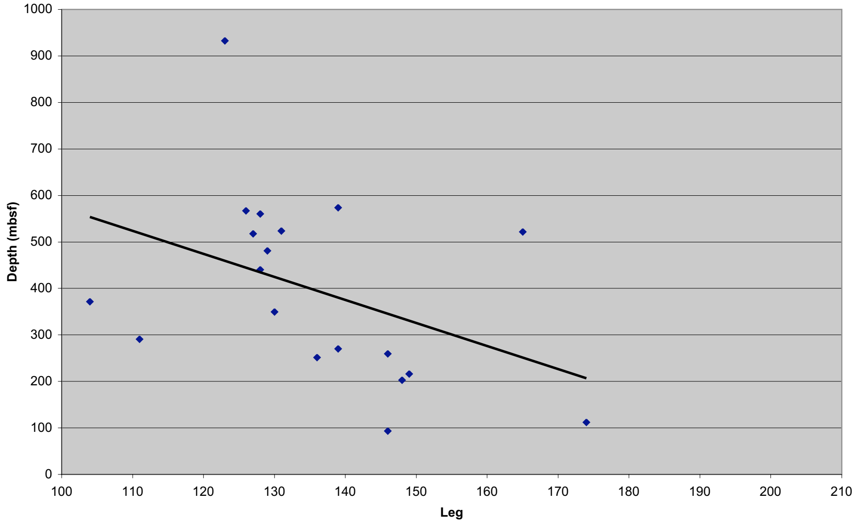
Depth of 11 3/4" Casings
